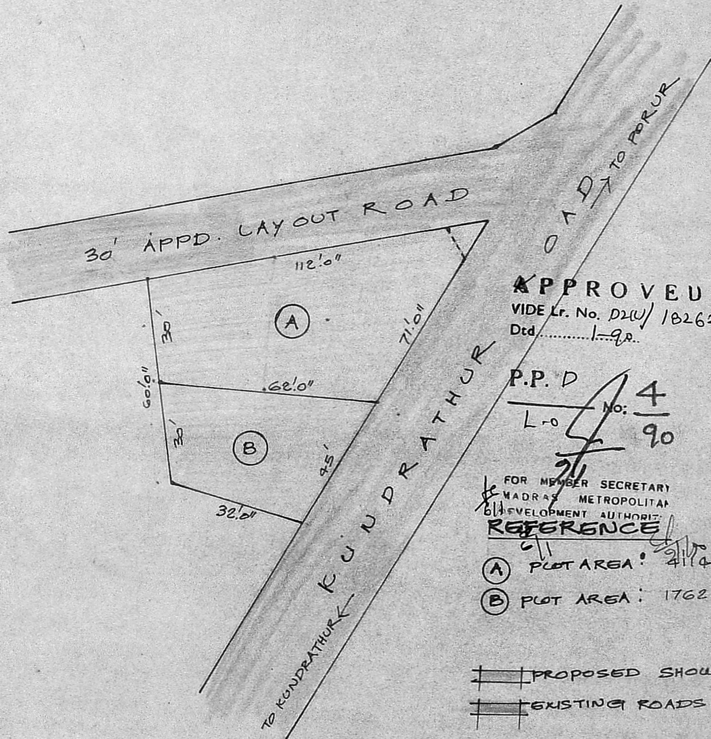
SUB-DIVISION PLAN
